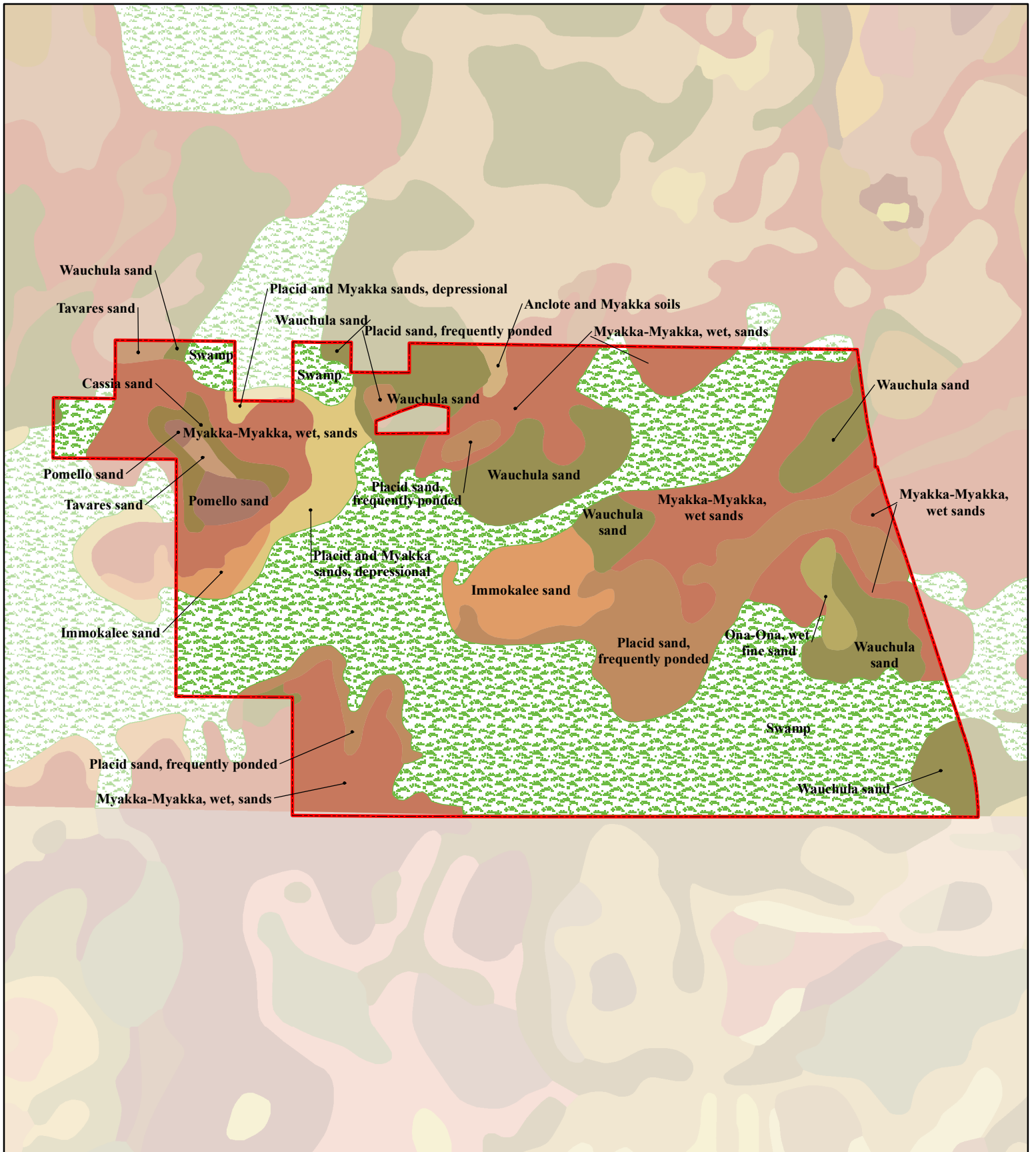
Figure 8 Soils Map
